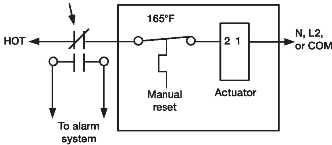
Auxiliary Switch Wiring
